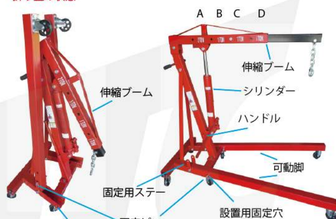
JTC2001C 2ton
